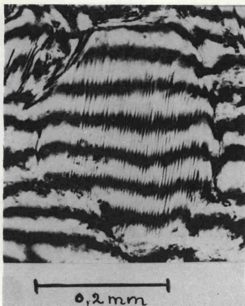
Fig. 8. Non-decorated planar elements in quartz. Two-ray-interference microscope (Leitz).
