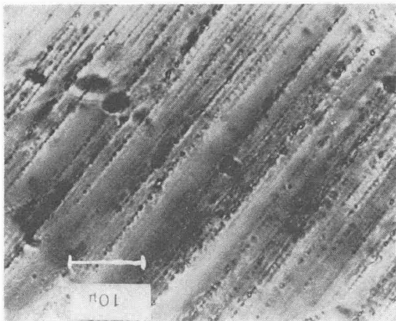
Fig. 6. Decorated planar elements in quartz. Granite inclusion, Zippelingen, Ries.
